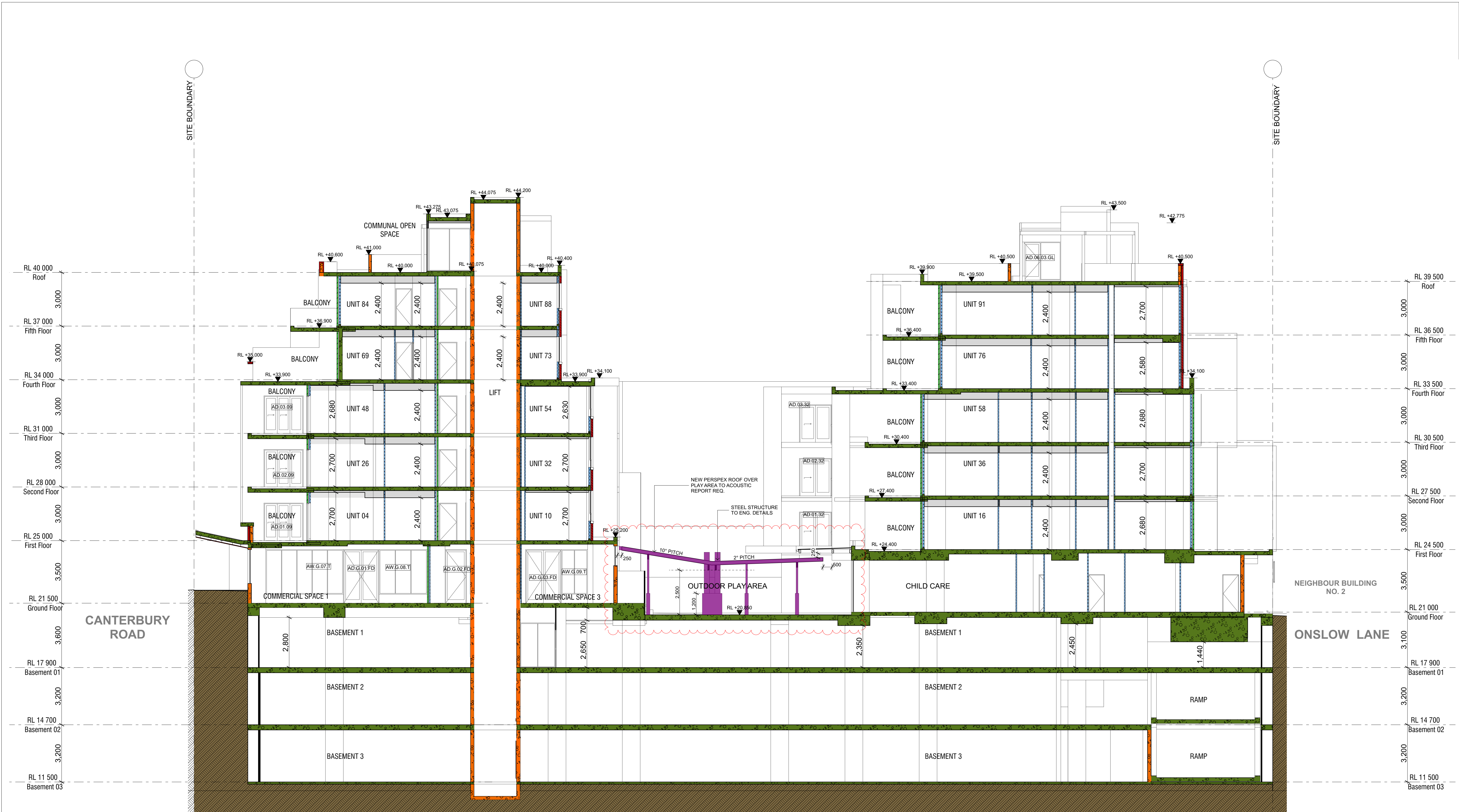
Section E 1:100
